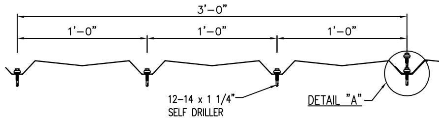
ALL MEMBER SCREW SPACING
